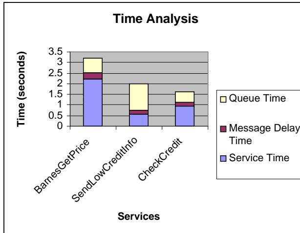
Figure 7. Performance: Time Analysis
