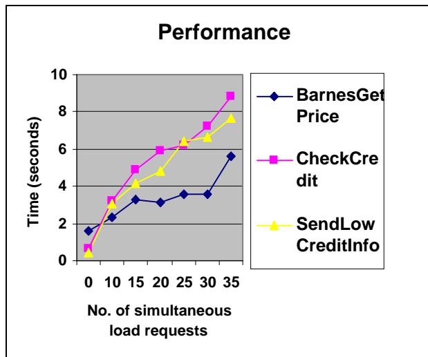
Figure 8. Load Testing Results for the Barnes Book Purchase Web Process
