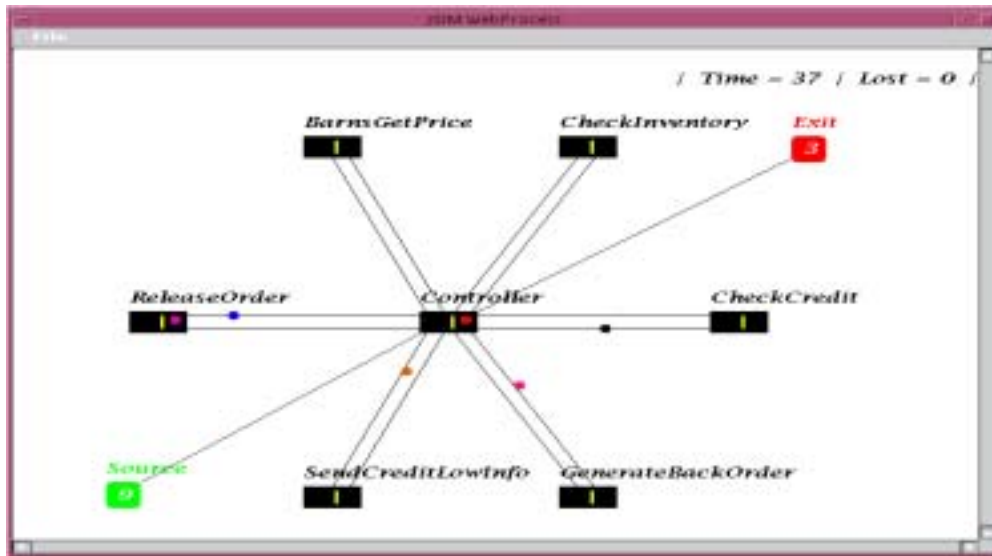
Figure 9. JSIM Centralized Execution Simulation
