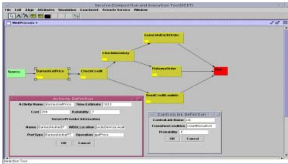
Figure 3. Web Process Composition using SCET
