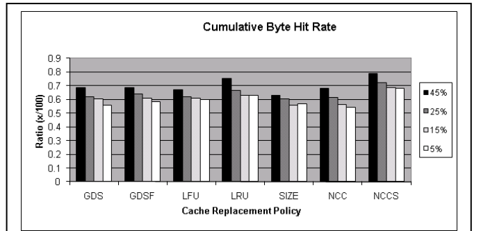
Figure 4. Cumulative Byte Hit Rate
