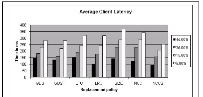
Figure 5. Average Client Latency
