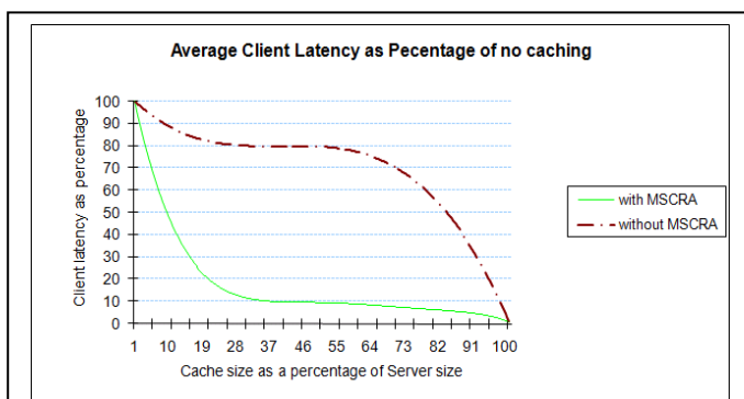
Figure 11. The average client latency calculated as the percentage of no-caching implementation with increasing total size of caching proxies as a percentage of total size of VPSs.
