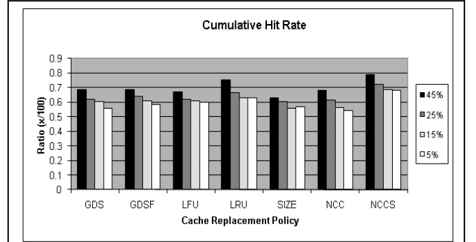
Figure 3. Cumulative Cache Hit Rate
