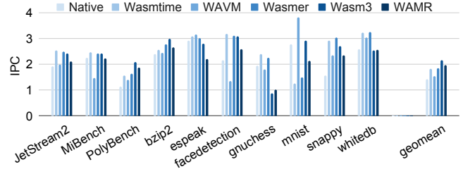
Figure 7: The instructions per cycle (IPC) of the native execution and WebAssembly runtimes.
