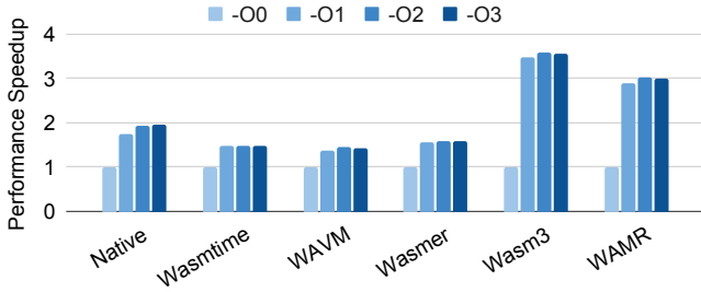
Figure 4: Performance speedup achieved by WebAssembly compiler optimizations. The baseline is -O0 . The results are geometric means of all benchmarks in WABench.
