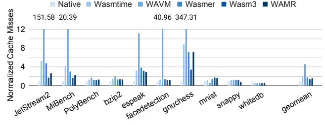
Figure 9: Normalized cache misses of WebAssembly runtimes. The baseline is the native execution.
