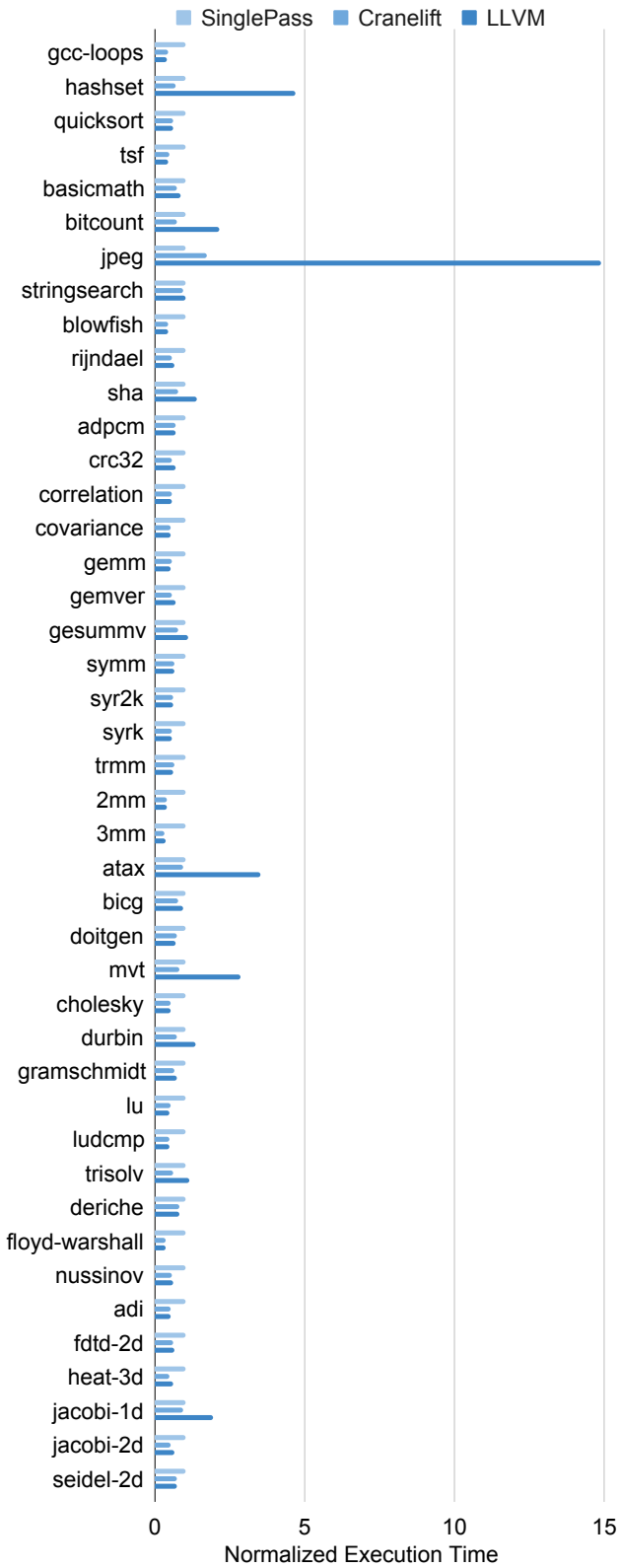
Figure 11: The normalized execution times of Wasmer with different JIT compilers for benchmarks from JetStream2, MiBench, and PolyBench. The baseline is SinglePass.
